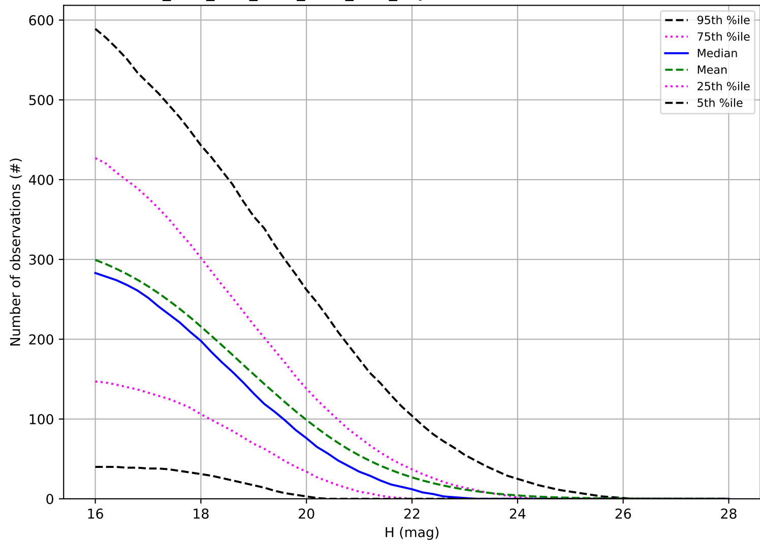
ddf_acor_sf20_lsf30_lsr20_v3.4_10yrs: Number of observations PHA
