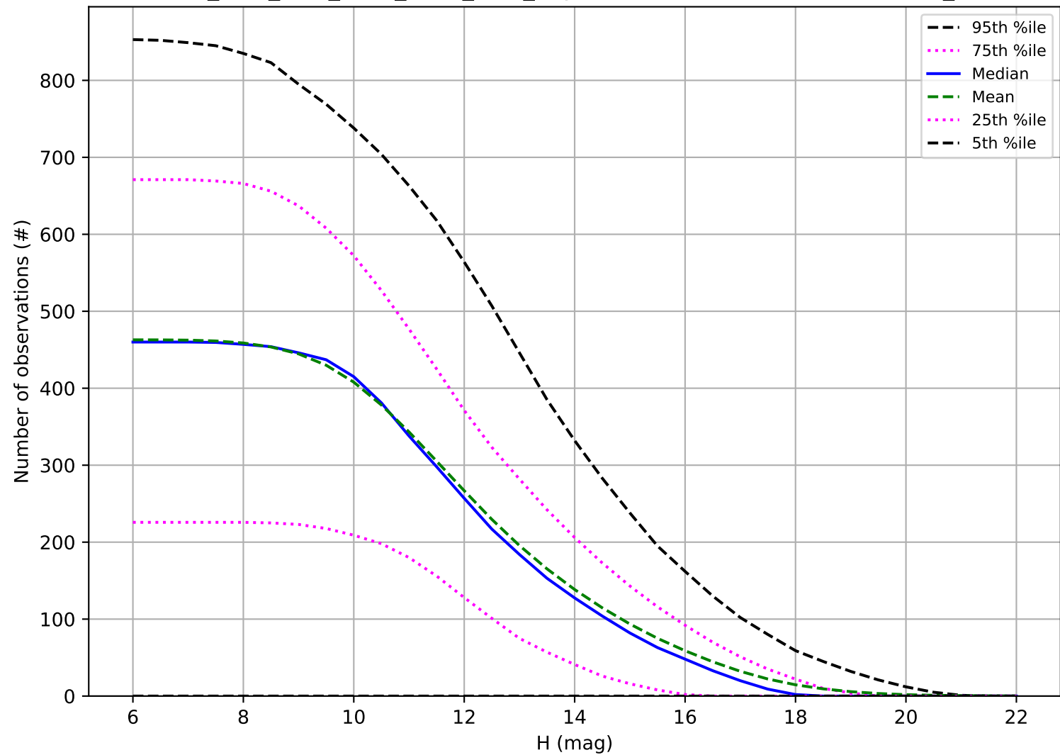
ddf_acor_sf20_lsf30_lsr20_v3.4_10yrs: Number of observations OCC_r5
