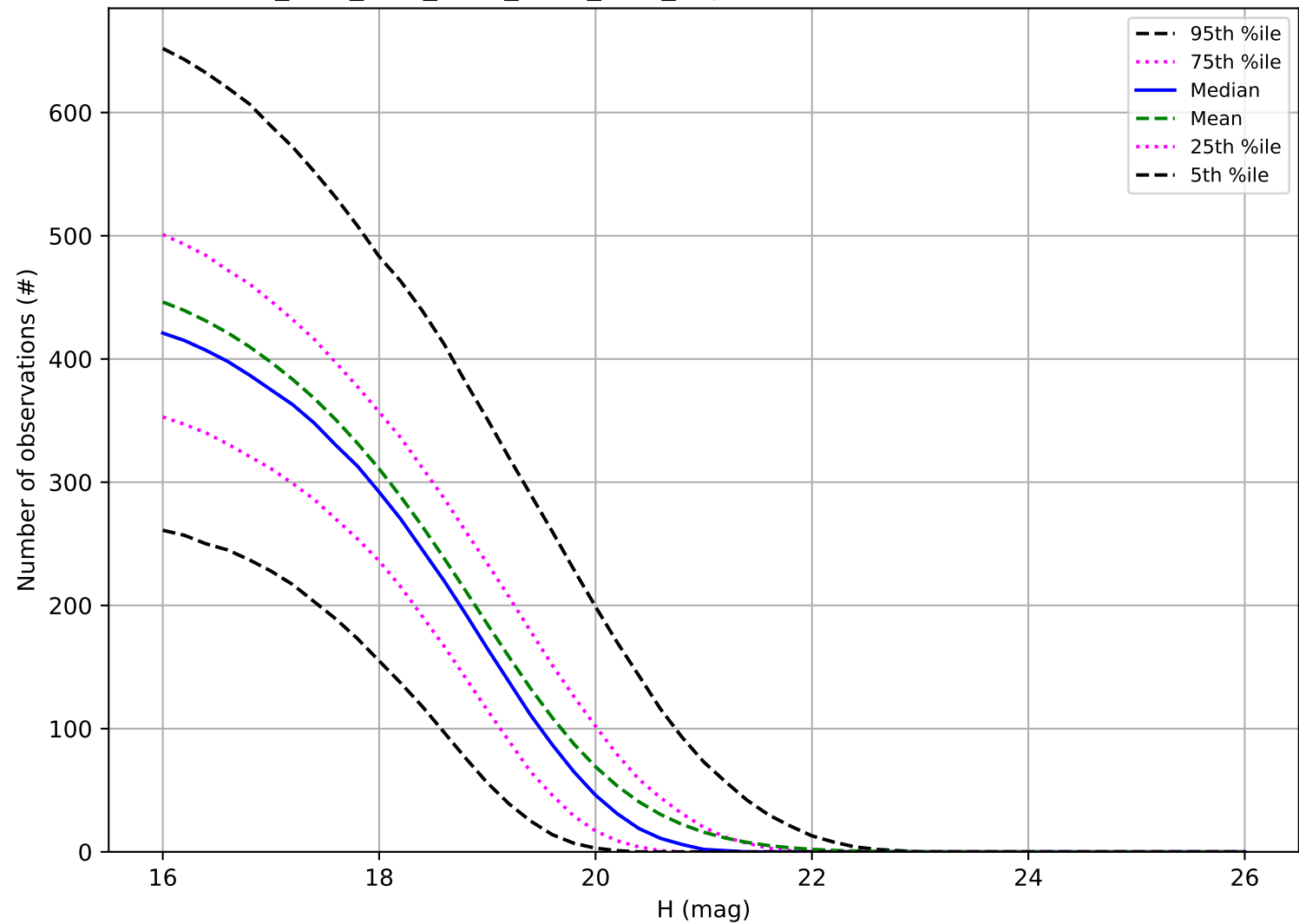
ddf_acor_sf20_lsf30_lsr20_v3.4_10yrs: Number of observations MBA
