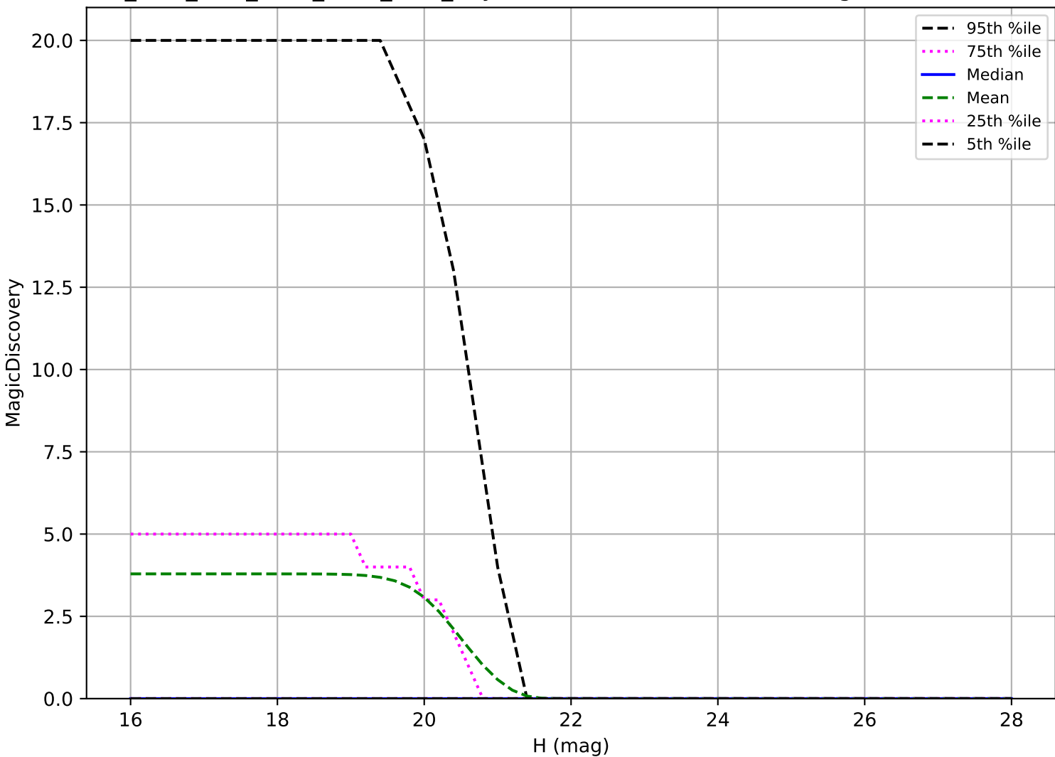
ddf_acor_sf20_lsf30_lsr20_v3.4_10yrs: Vatra 6 detections in 60 nights detection loss
