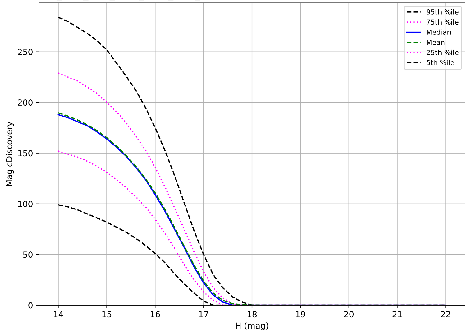
ddf_acor_sf20_lsf30_lsr20_v3.4_10yrs: Trojan 6 detections in 60 nights detection loss
