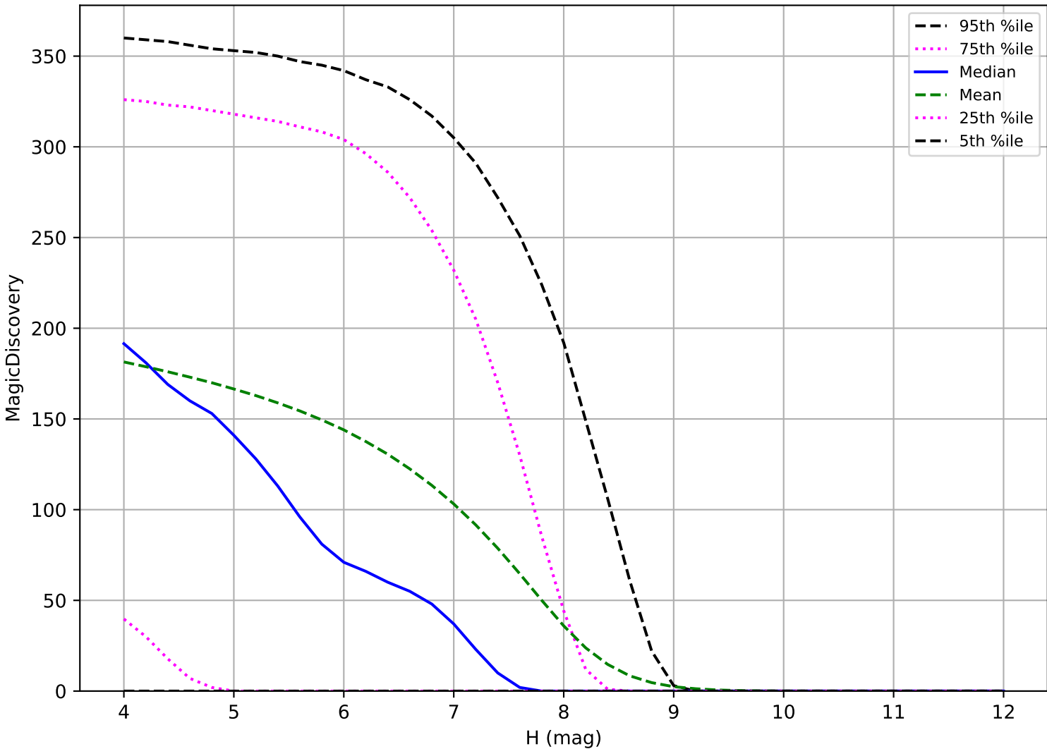
ddf_acor_sf20_lsf30_lsr20_v3.4_10yrs: TNO 6 detections in 60 nights detection loss
