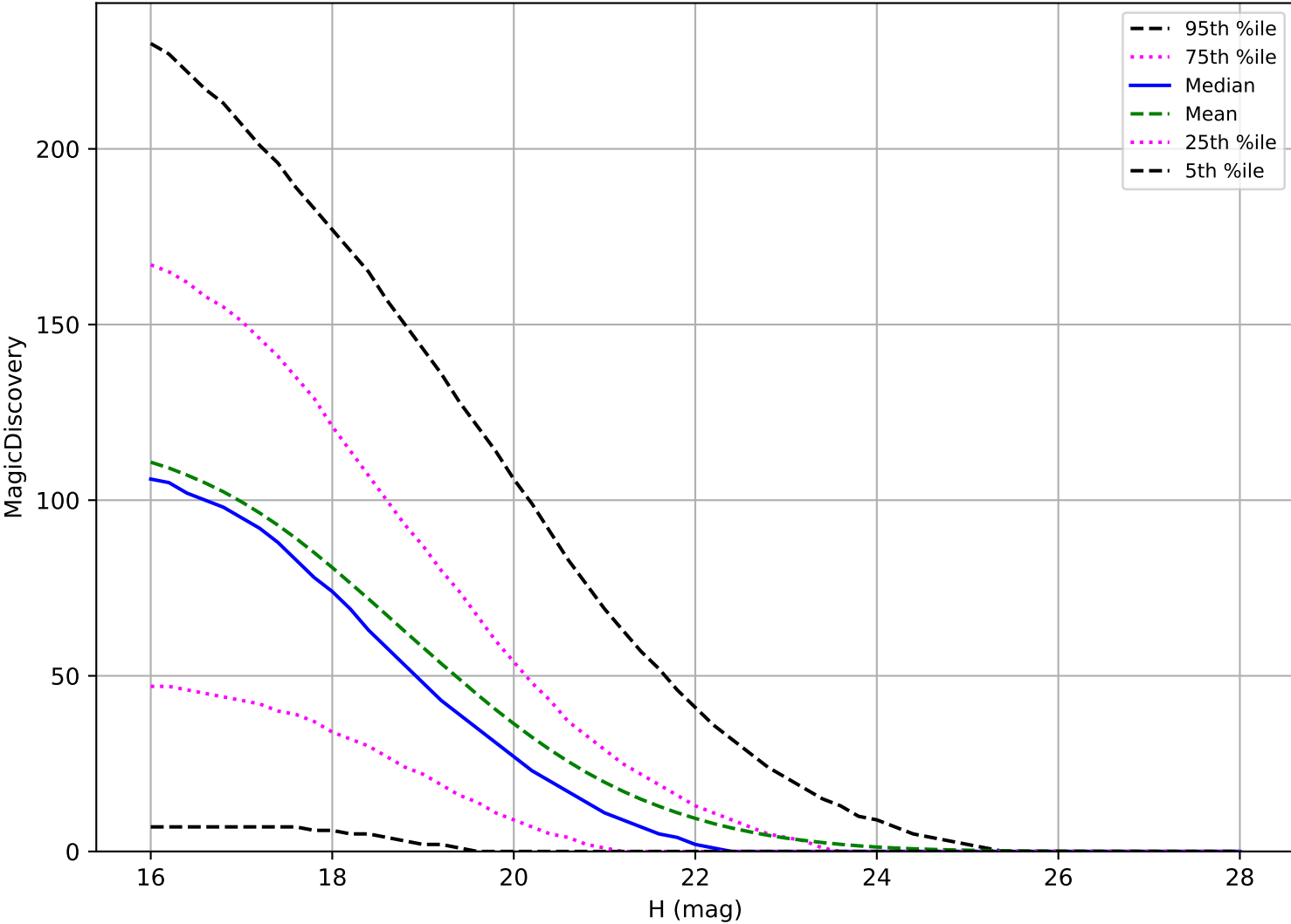
ddf_acor_sf20_lsf30_lsr20_v3.4_10yrs: PHA 6 detections in 60 nights detection loss
