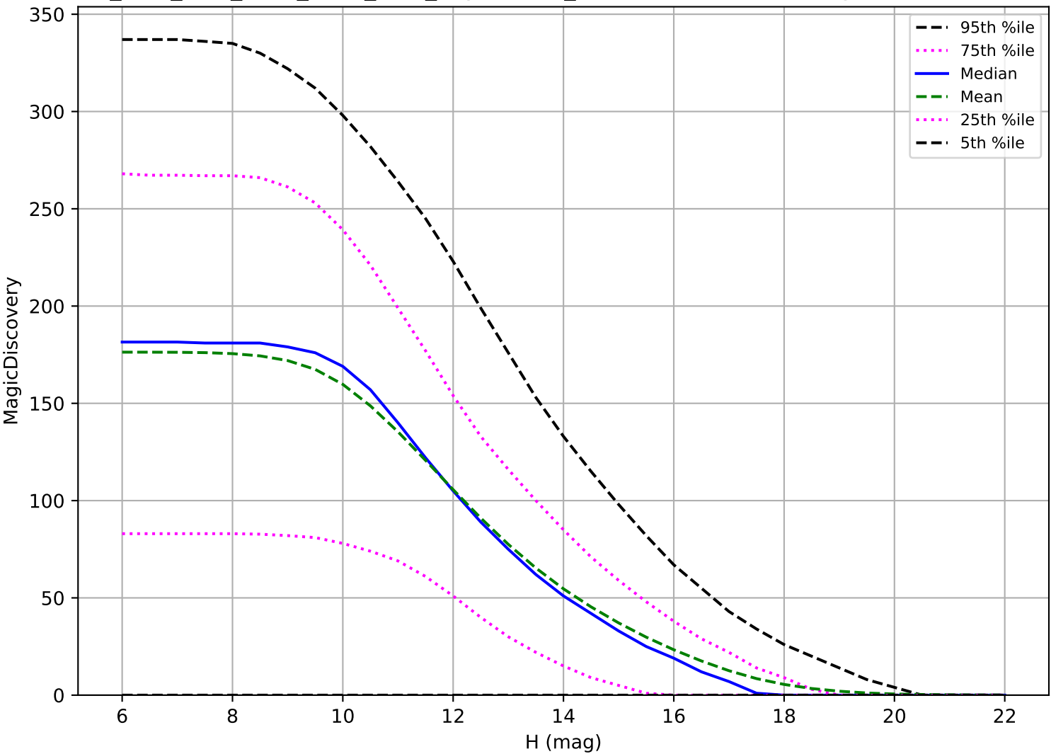
ddf_acor_sf20_lsf30_lsr20_v3.4_10yrs: OCC_r5 6 detections in 60 nights detection loss
