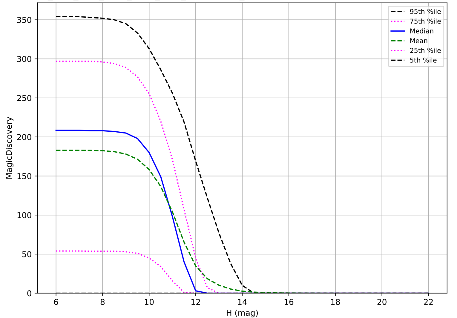
ddf_acor_sf20_lsf30_lsr20_v3.4_10yrs: OCC_r20 6 detections in 60 nights detection loss
