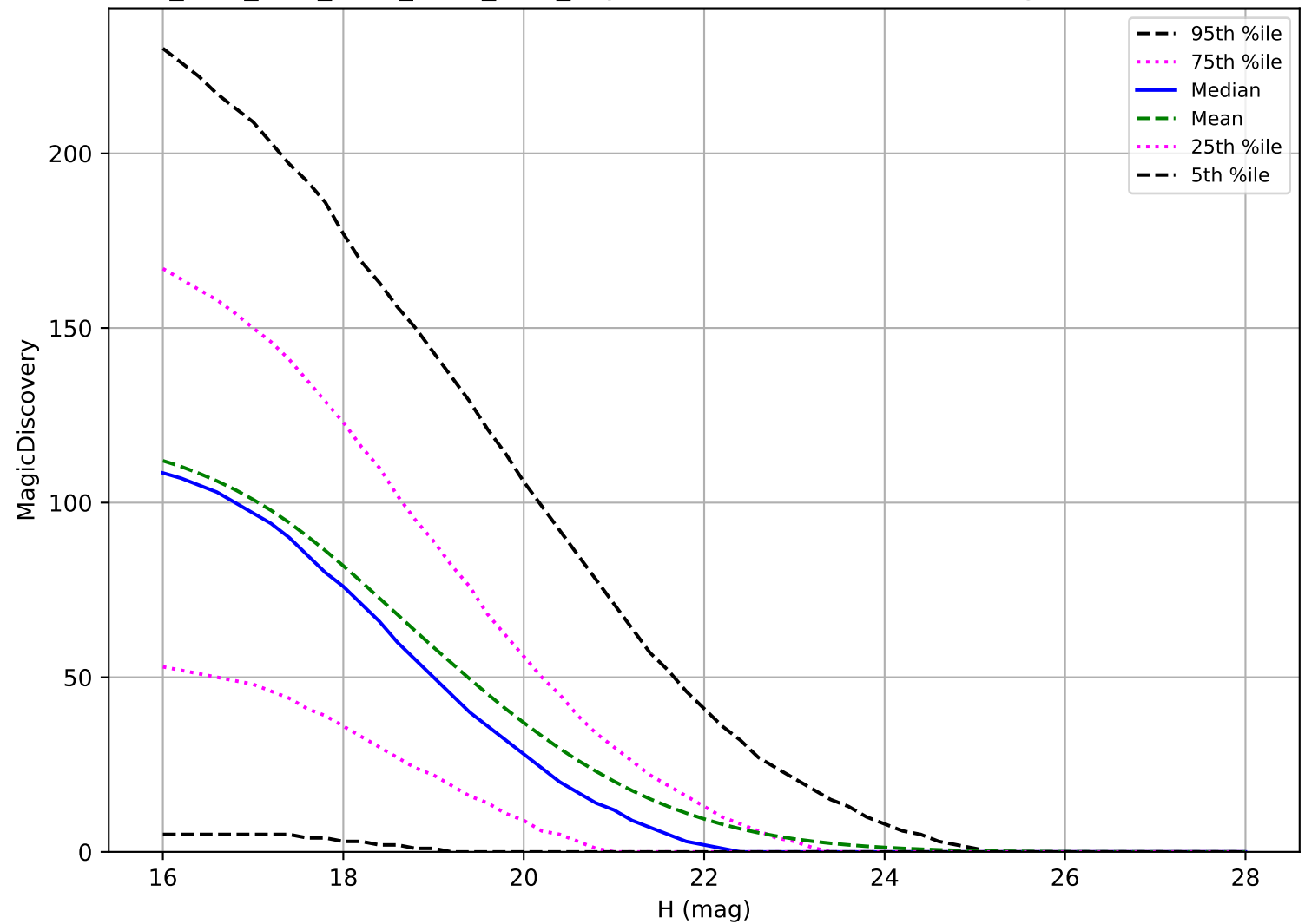
ddf_acor_sf20_lsf30_lsr20_v3.4_10yrs: NEO 6 detections in 60 nights detection loss
