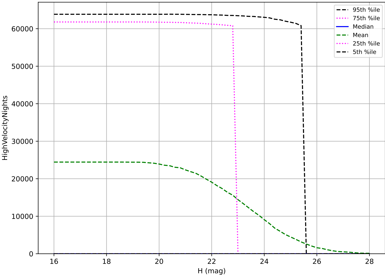
ddf_acor_sf20_lsf30_lsr20_v3.4_10yrs: PHA High velocity pair detection loss
