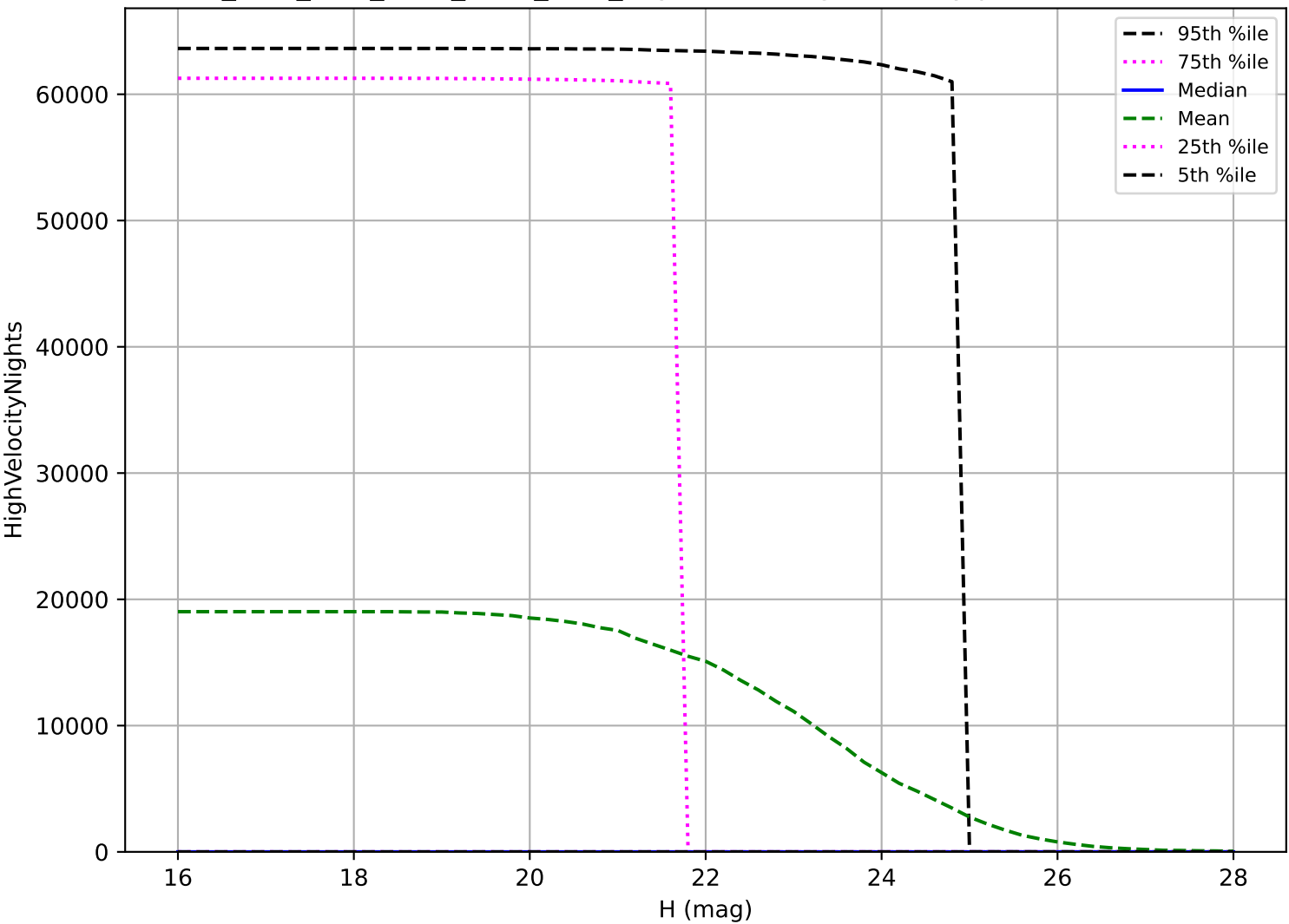
ddf_acor_sf20_lsf30_lsr20_v3.4_10yrs: NEO High velocity pair detection loss
