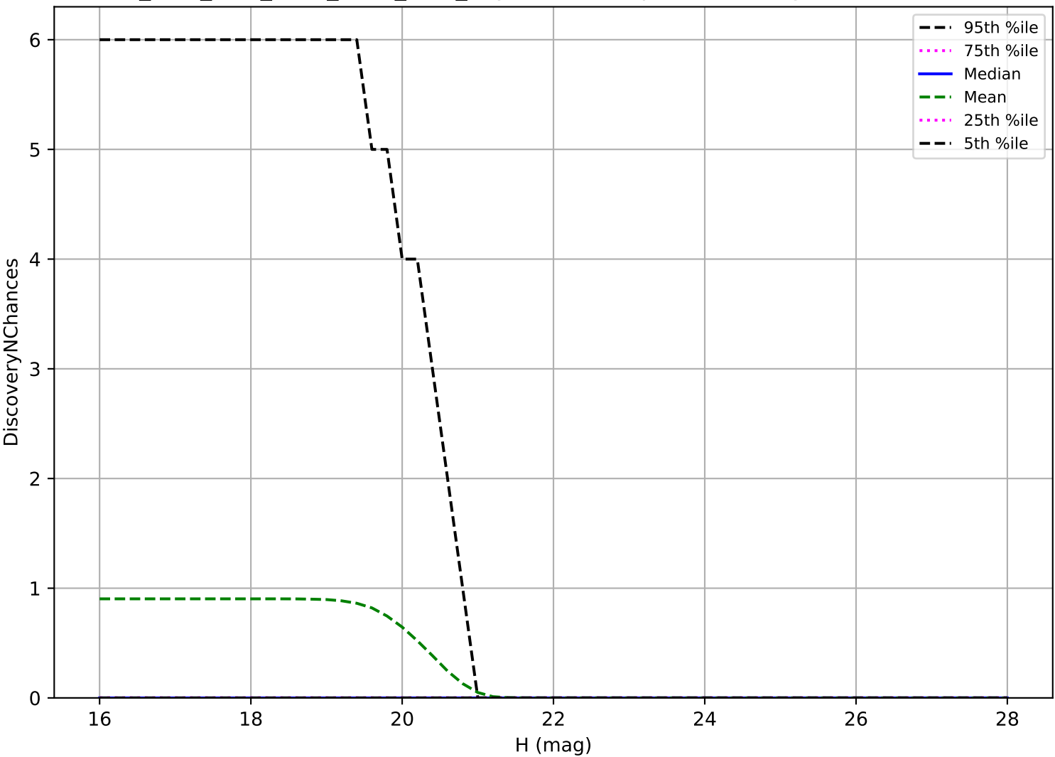
ddf_acor_sf20_lsf30_lsr20_v3.4_10yrs: Vatira 3 pairs in 15 nights detection loss
