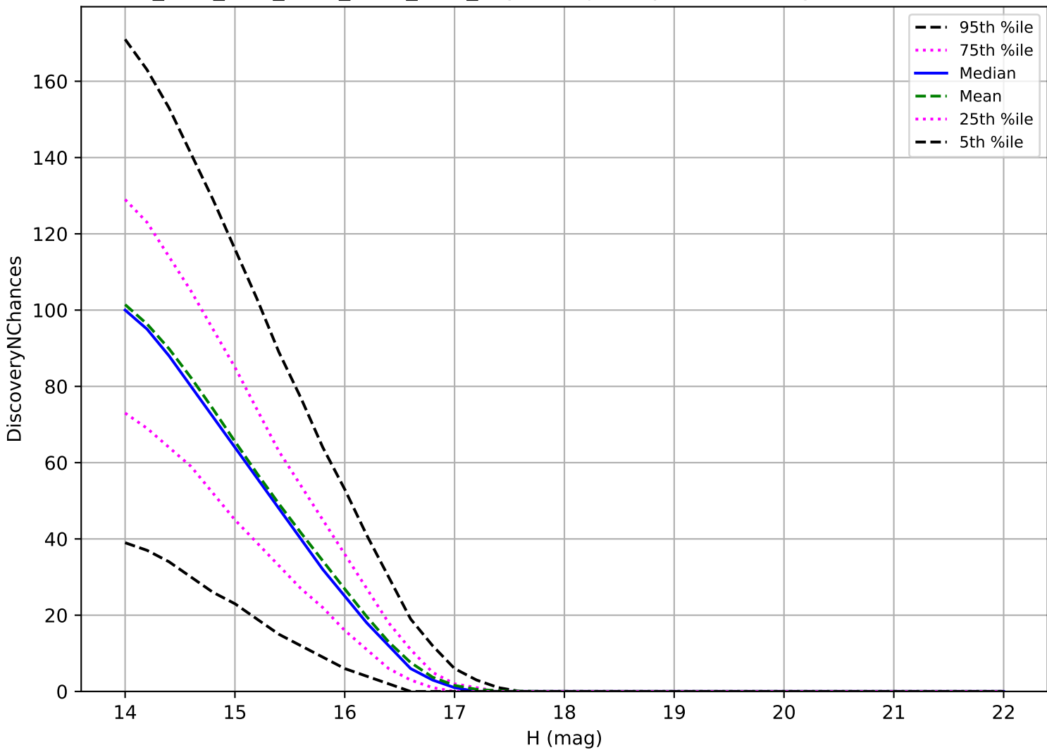
ddf_acor_sf20_lsf30_lsr20_v3.4_10yrs: Trojan 3 pairs in 15 nights detection loss
