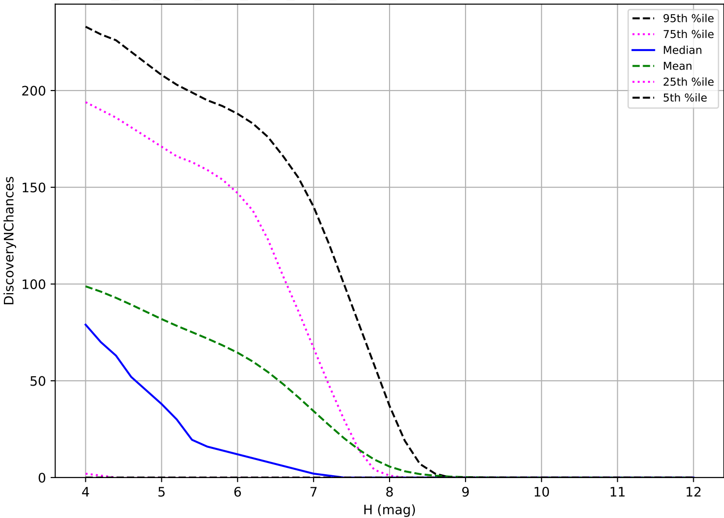
ddf_acor_sf20_lsf30_lsr20_v3.4_10yrs: TNO 3 pairs in 15 nights detection loss
