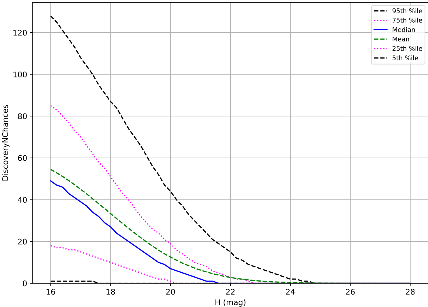
ddf_acor_sf20_lsf30_lsr20_v3.4_10yrs: PHA 3 pairs in 15 nights detection loss
