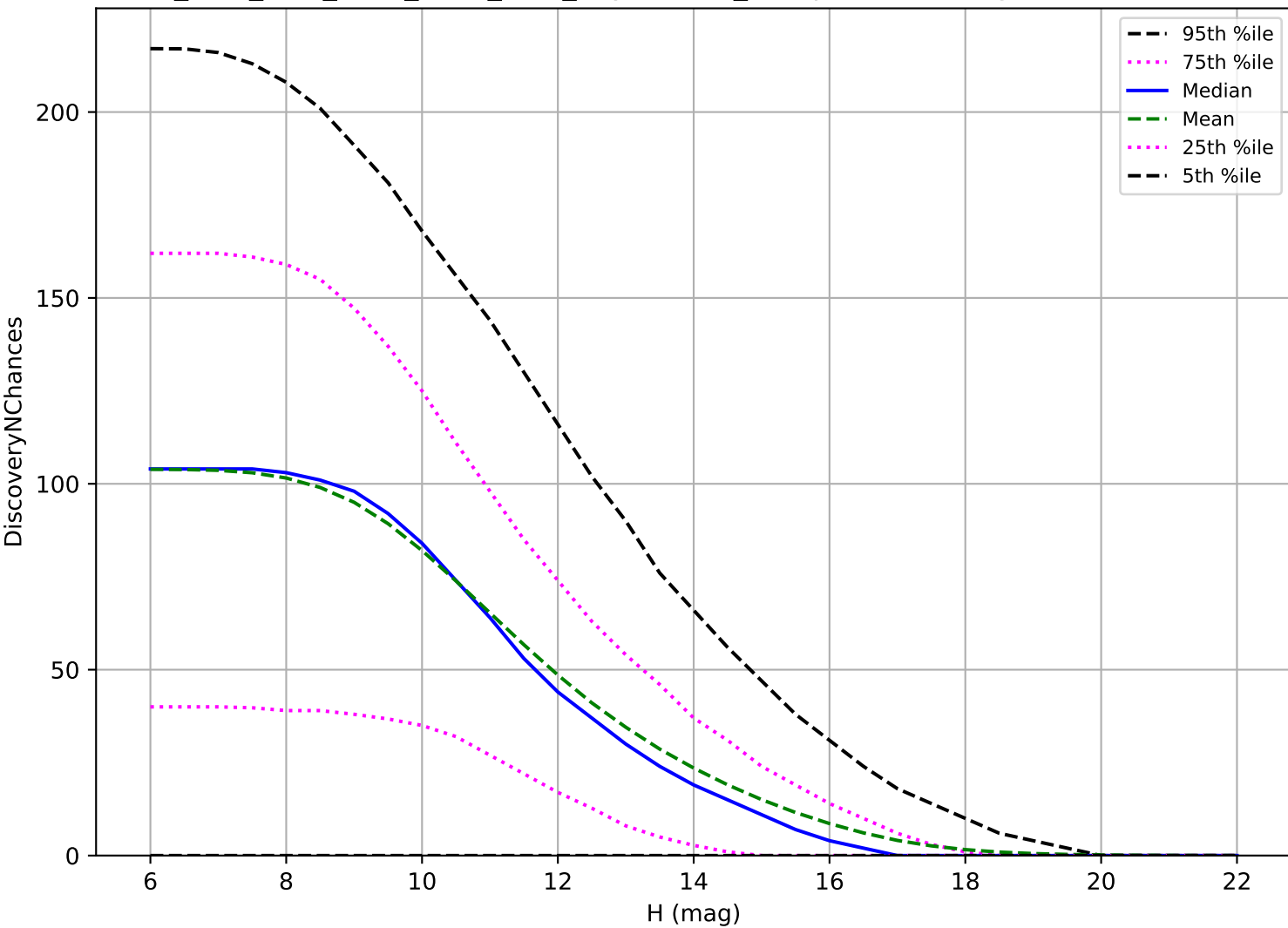
ddf_acor_sf20_lsf30_lsr20_v3.4_10yrs: OCC_r5 3 pairs in 15 nights detection loss
