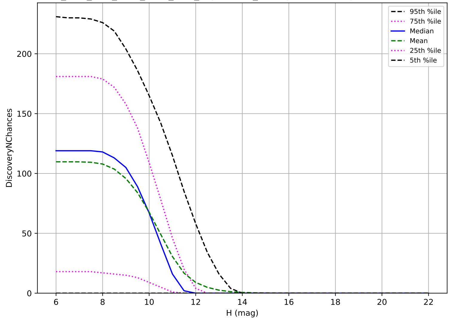
ddf_acor_sf20_lsf30_lsr20_v3.4_10yrs: OCC_r20 3 pairs in 15 nights detection loss
