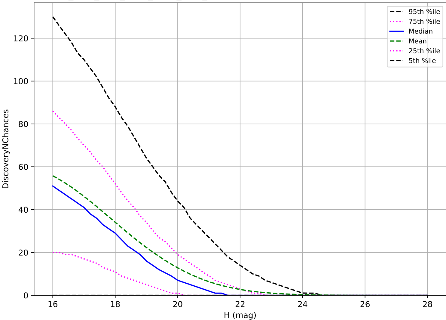
ddf_acor_sf20_lsf30_lsr20_v3.4_10yrs: NEO 3 pairs in 15 nights detection loss
