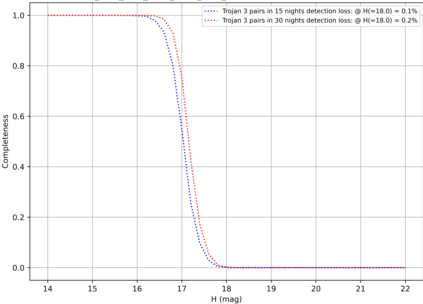
ddf_acor_sf20_lsf30_lsr20_v3.4_10yrs: DifferentialCompleteness
