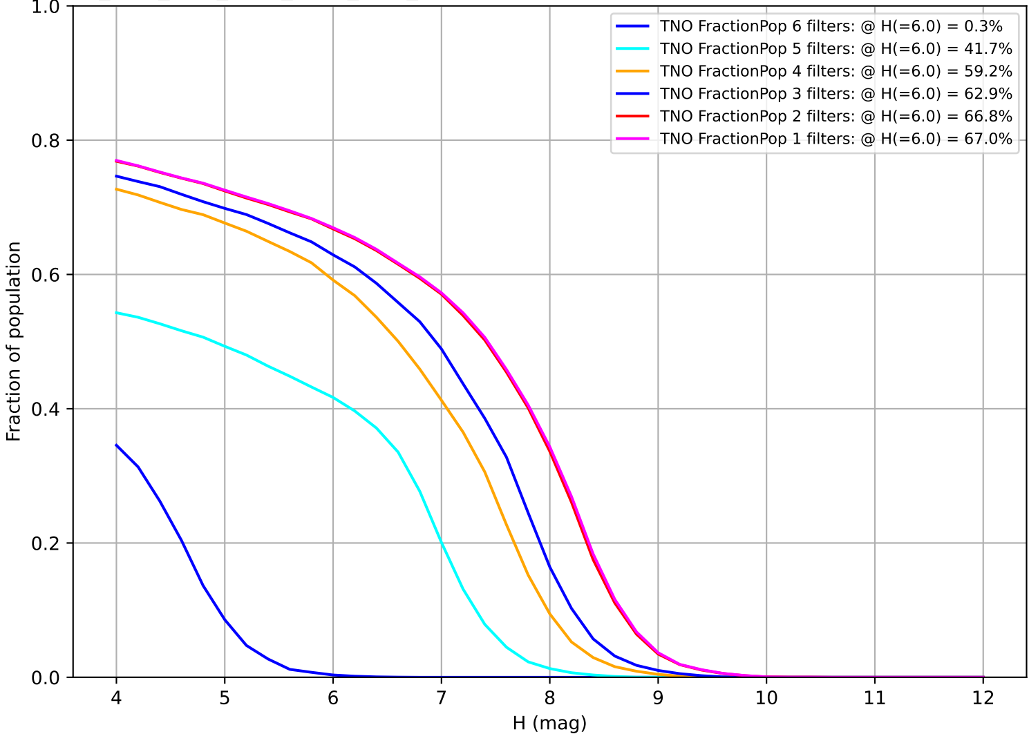
ddf_acor_sf20_lsf30_lsr20_v3.4_10yrs: Fraction of population with colors in X filters TNO
