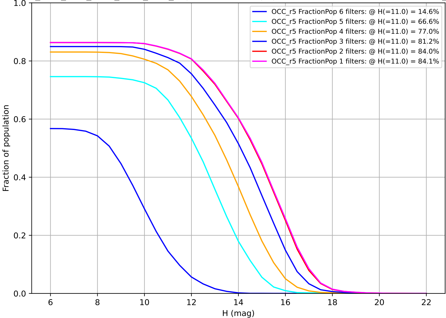
ddf_acor_sf20_lsf30_lsr20_v3.4_10yrs: Fraction of population with colors in X filters OCC_r5
