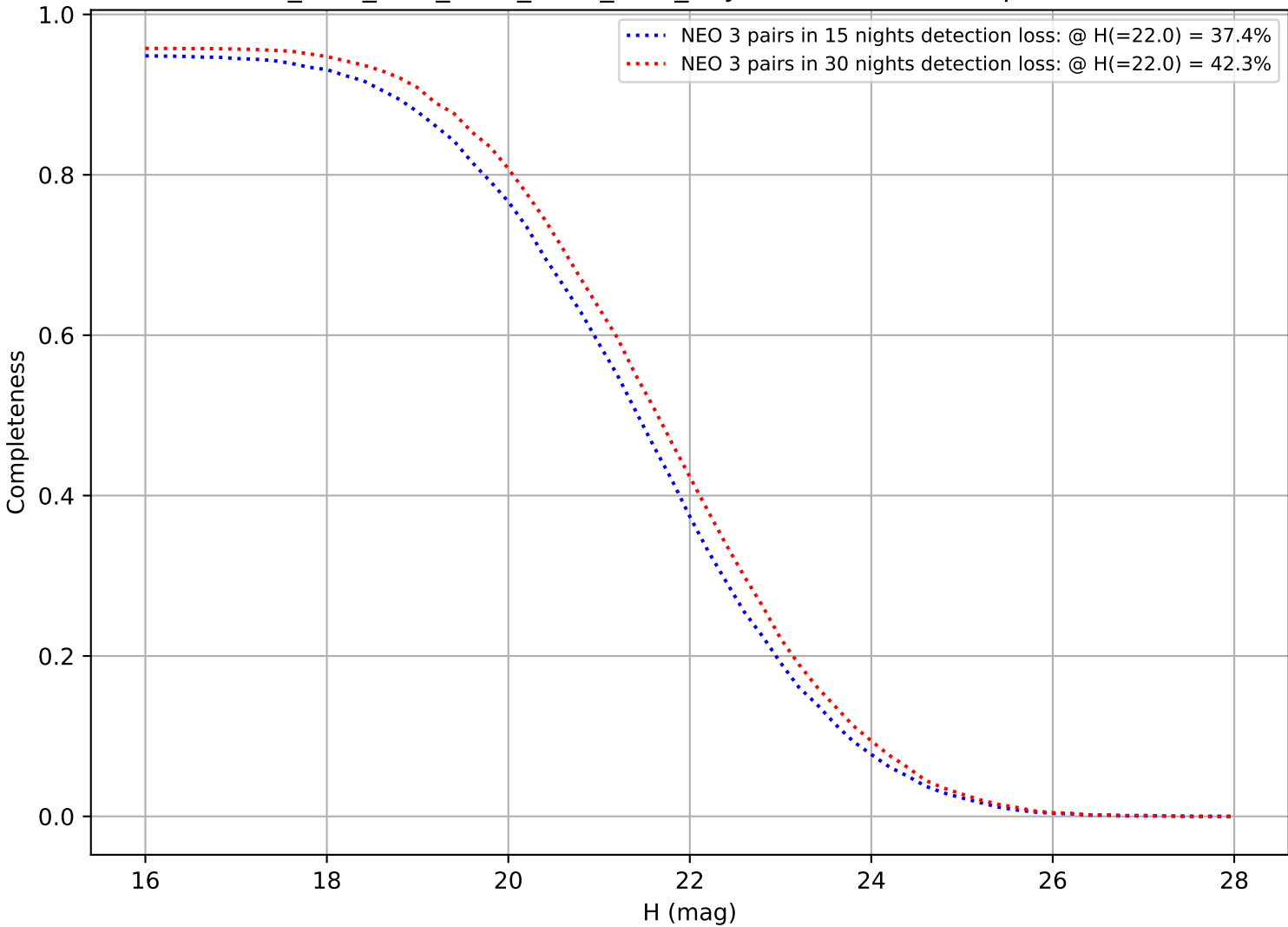
ddf_acor_sf20_lsf30_lsr20_v3.4_10yrs: DifferentialCompleteness
