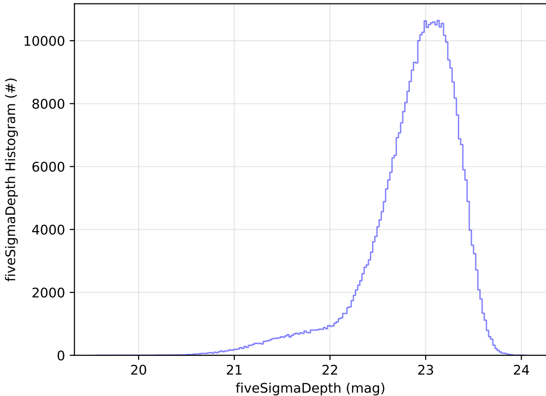
ddf_acor_sf20_lsf30_lsr20_v3.4_10yrs z: fiveSigmaDepth Histogram
