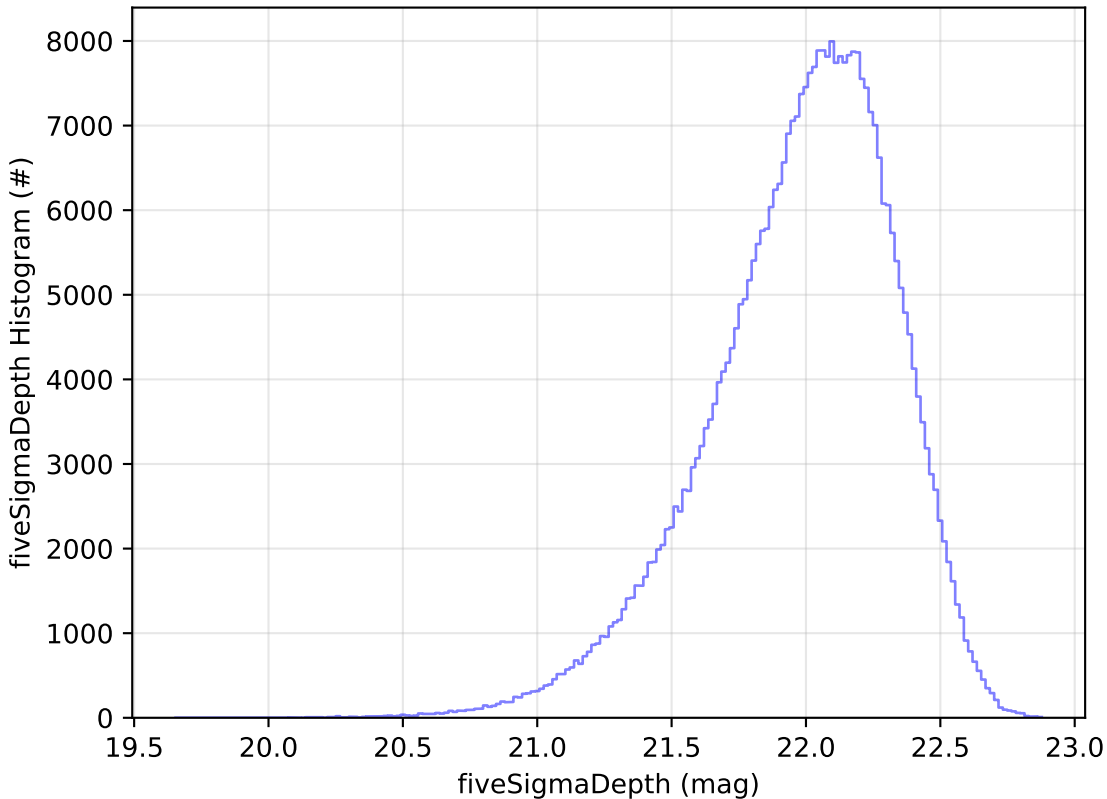
ddf_acor_sf20_lsf30_lsr20_v3.4_10yrs y: fiveSigmaDepth Histogram
