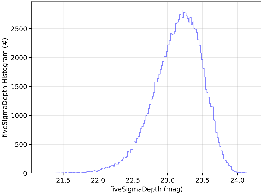
ddf_acor_sf20_lsf30_lsr20_v3.4_10yrs u: fiveSigmaDepth Histogram
