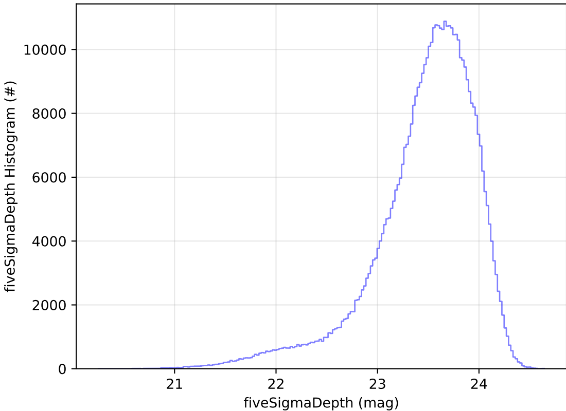
ddf_acor_sf20_lsf30_lsr20_v3.4_10yrs i: fiveSigmaDepth Histogram
