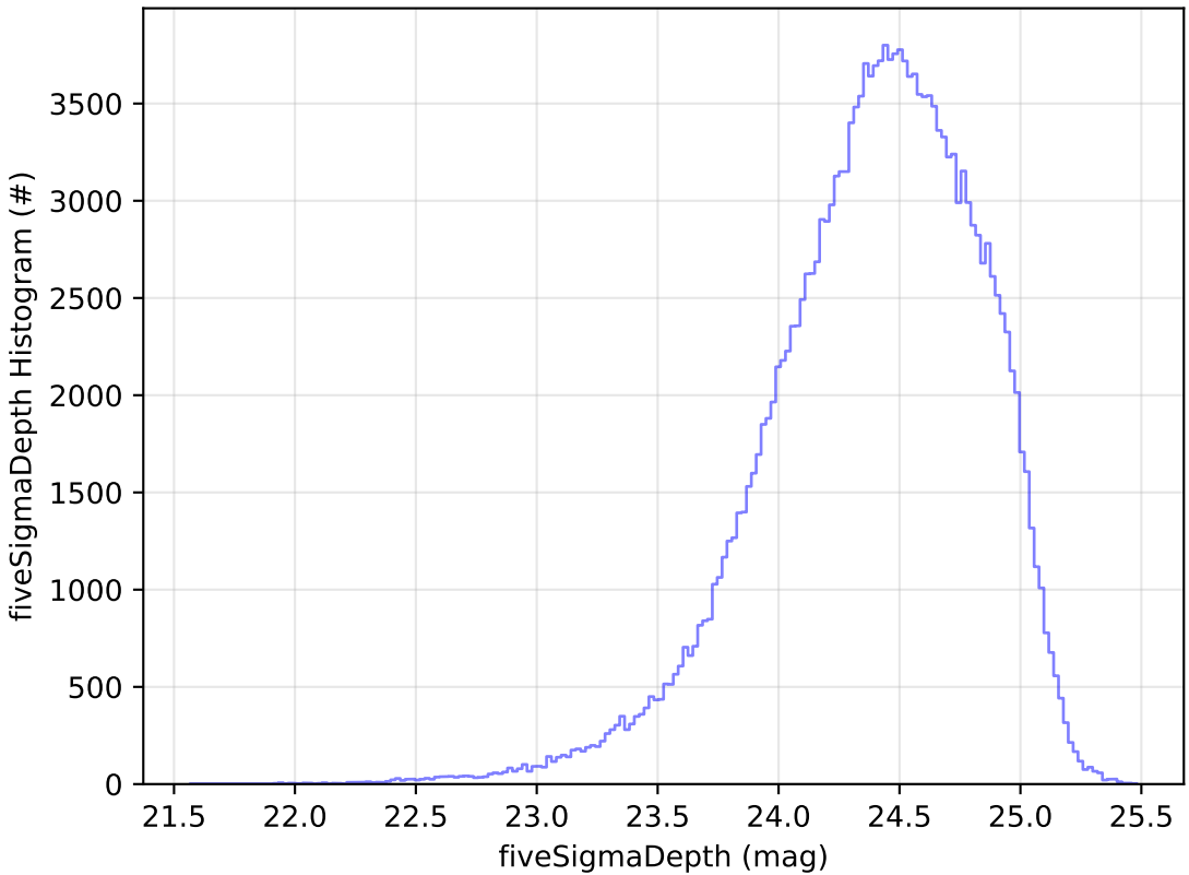
ddf_acor_sf20_lsf30_lsr20_v3.4_10yrs g: fiveSigmaDepth Histogram
