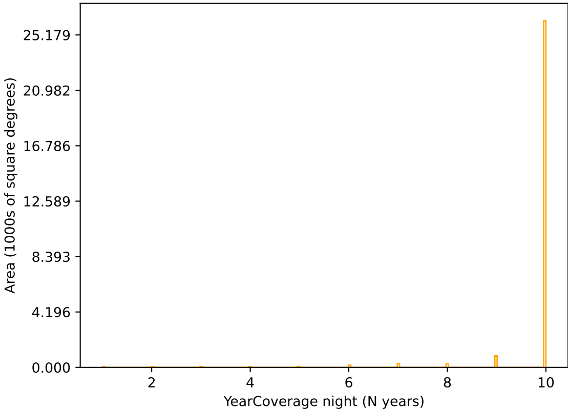
ddf_acor_sf20_lsf30_lsr20_v3.4_10yrs r band: YearCoverage night
