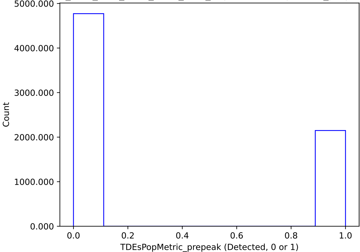
ddf_acor_sf20_lsf30_lsr20_v3.4_10yrs : TDEsPopMetric_prepeak
