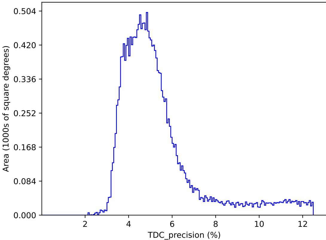
ddf_acor_sf20_lsf30_lsr20_v3.4_10yrs : TDC_precision
