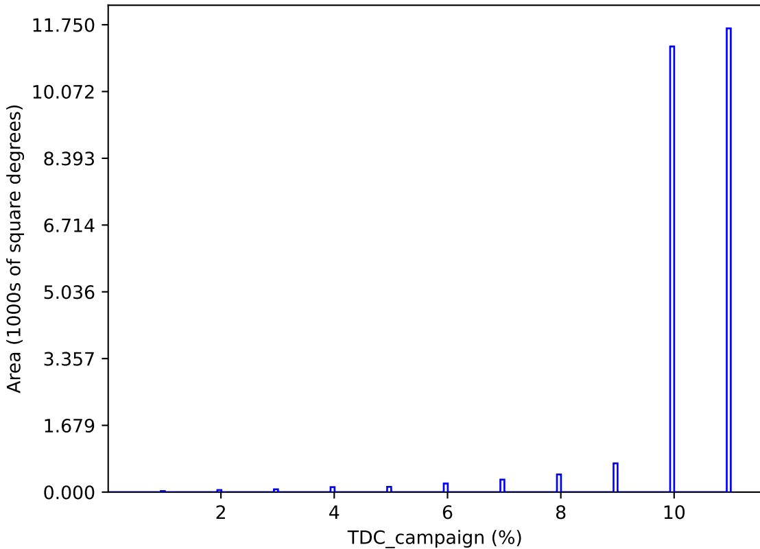
ddf_acor_sf20_lsf30_lsr20_v3.4_10yrs : TDC_campaign
