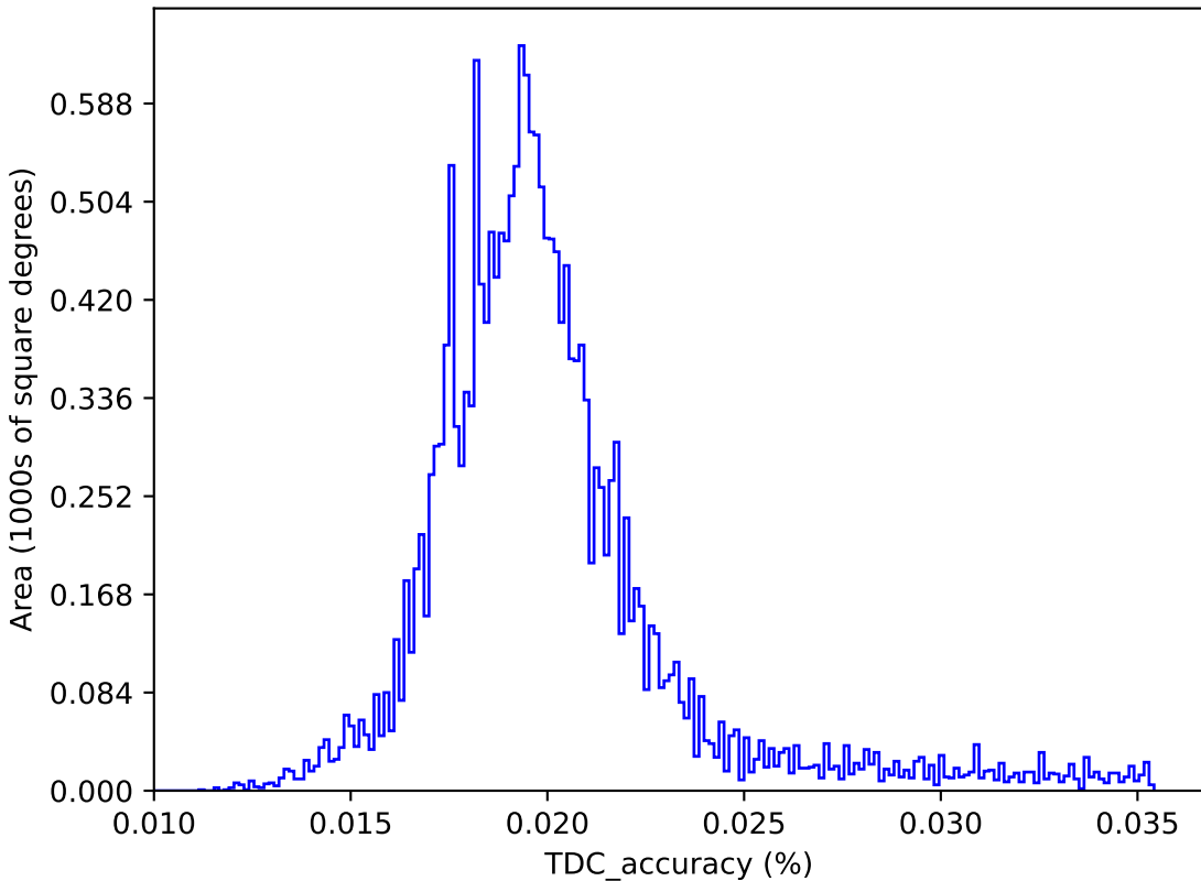
ddf_acor_sf20_lsf30_lsr20_v3.4_10yrs : TDC_accuracy
