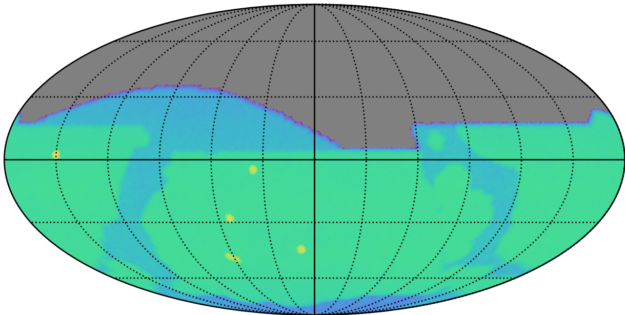
ddf_acor_sf20_lsf30_lsr20_v3.4_10yrs i: SurfaceBrightLimit
