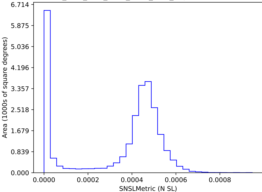
ddf_acor_sf20_lsf30_lsr20_v3.4_10yrs : SNSLMetric
