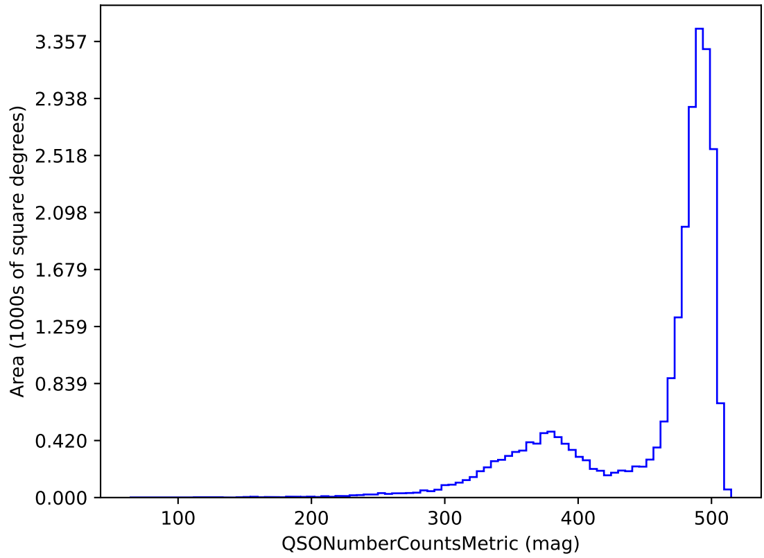
ddf_acor_sf20_lsf30_lsr20_v3.4_10yrs z band and non-DD: QSONumberCountsMetric
