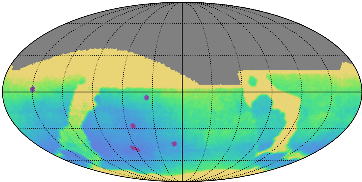
ddf_acor_sf20_lsf30_lsr20_v3.4_10yrs : Parallax Uncert @ 24.0
