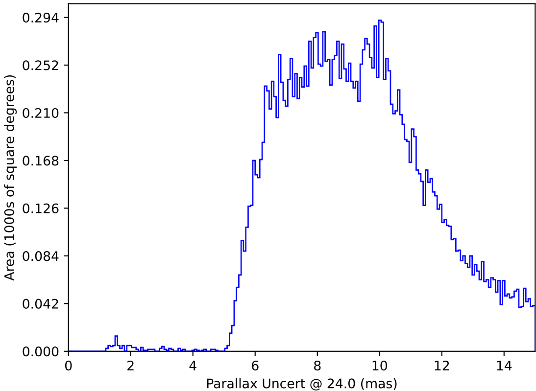
ddf_acor_sf20_lsf30_lsr20_v3.4_10yrs : Parallax Uncert @ 24.0
