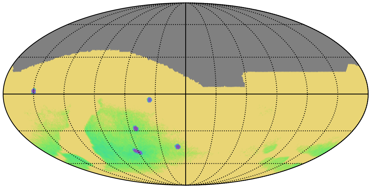
ddf_acor_sf20_lsf30_lsr20_v3.4_10yrs : Parallax Uncert @ 22.4
