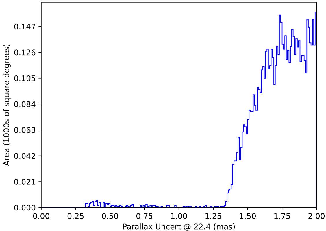
ddf_acor_sf20_lsf30_lsr20_v3.4_10yrs : Parallax Uncert @ 22.4
