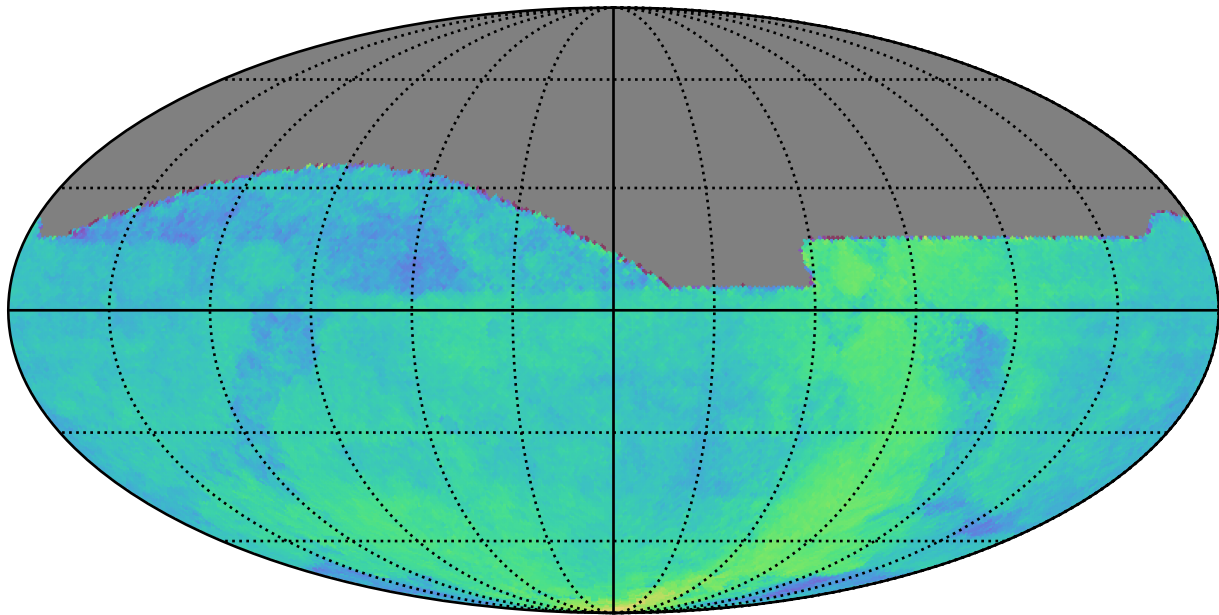
ddf_acor_sf20_lsf30_lsr20_v3.4_10yrs : Parallax Coverage @ 24.0
