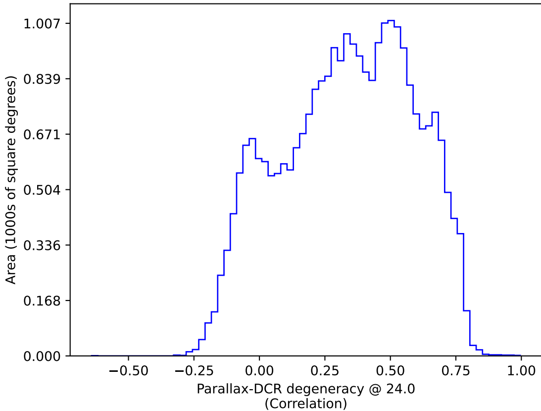
ddf_acor_sf20_lsf30_lsr20_v3.4_10yrs : Parallax-DCR degeneracy @ 24.0
