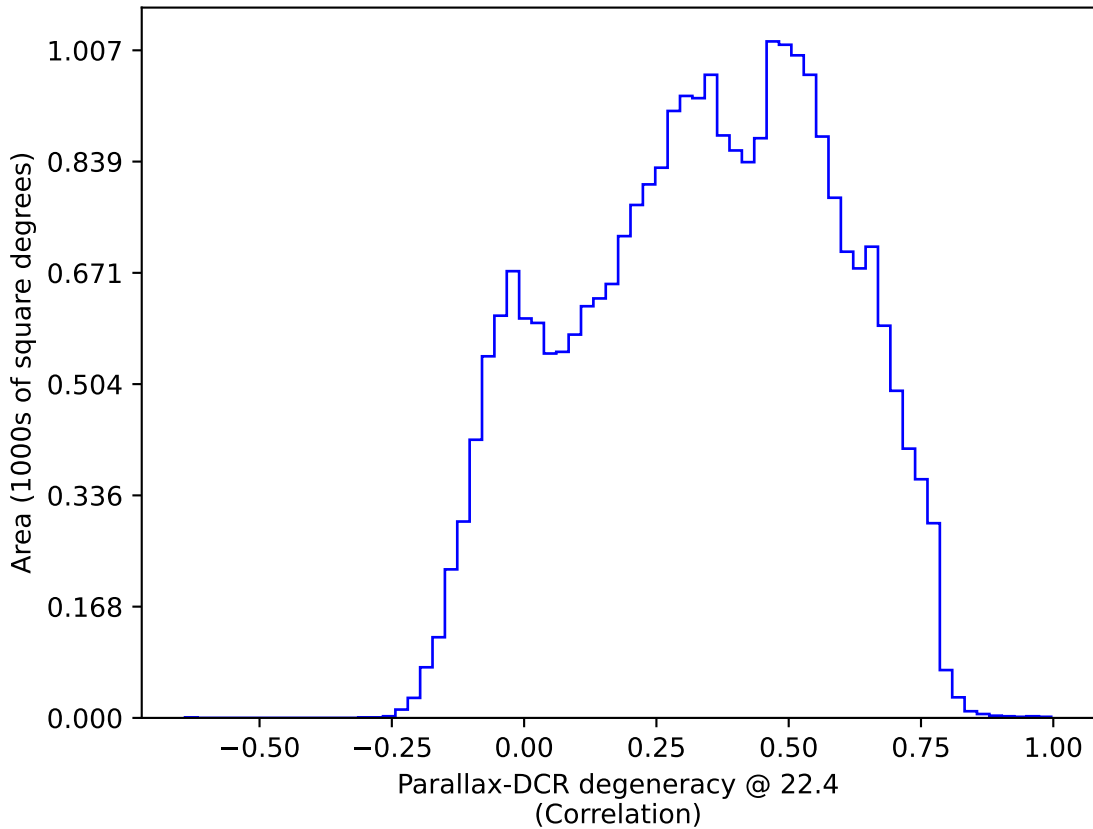
ddf_acor_sf20_lsf30_lsr20_v3.4_10yrs : Parallax-DCR degeneracy @ 22.4
