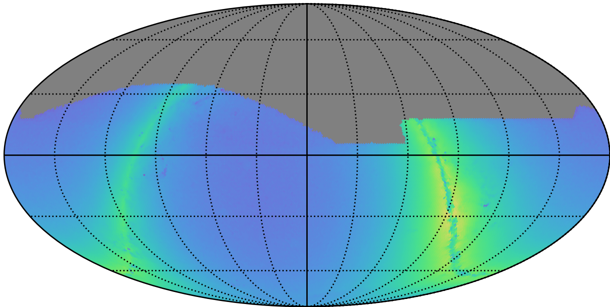
ddf_acor_sf20_lsf30_lsr20_v3.4_10yrs r: Nstars_no_crowding
