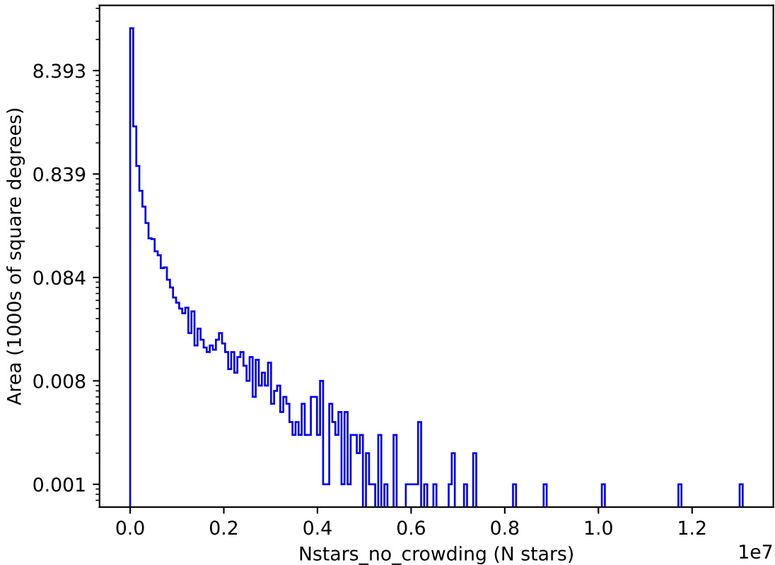
ddf_acor_sf20_lsf30_lsr20_v3.4_10yrs g: Nstars_no_crowding
