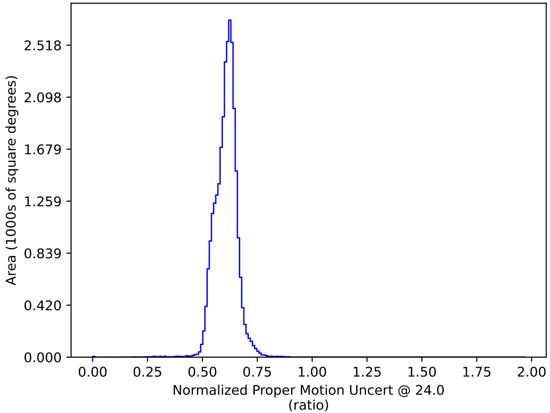
ddf_acor_sf20_lsf30_lsr20_v3.4_10yrs : Normalized Proper Motion Uncert @ 24.0
