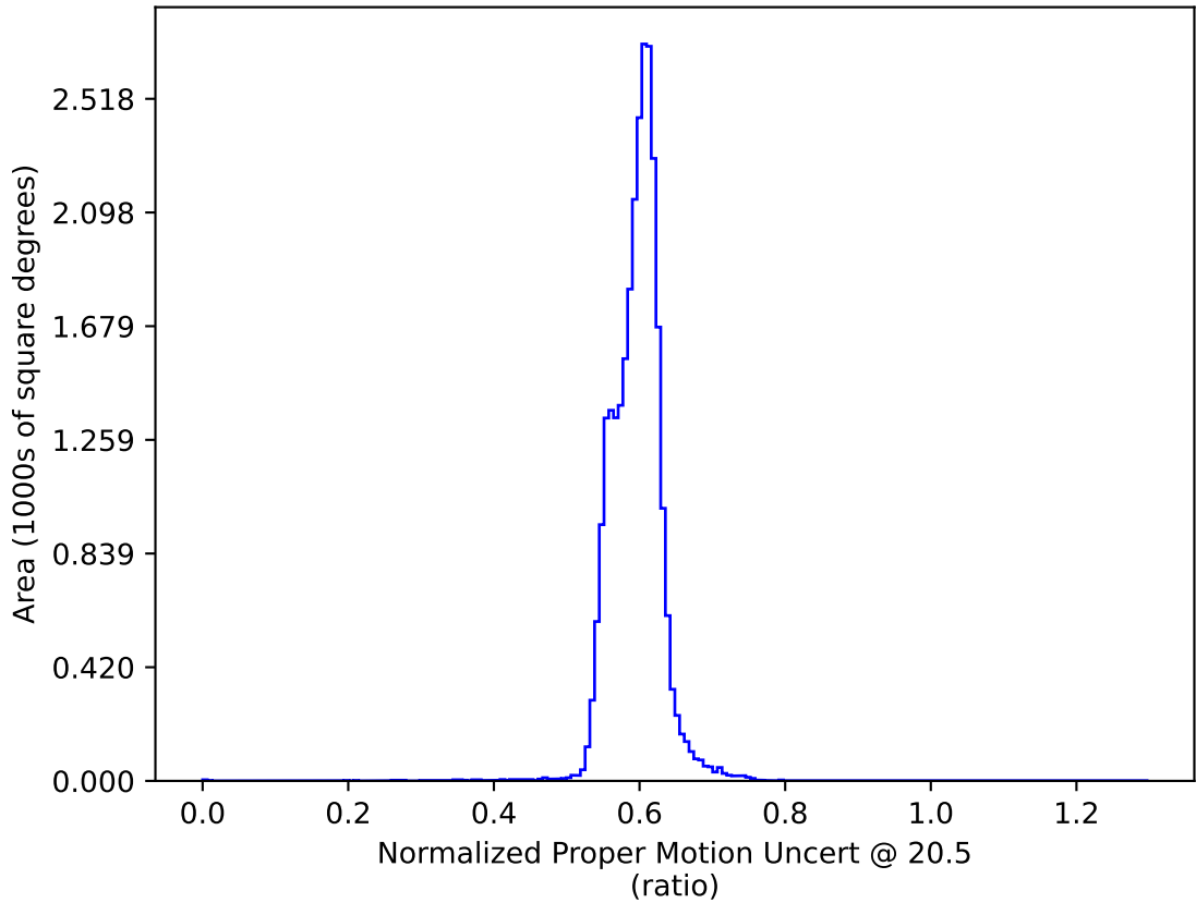
ddf_acor_sf20_lsf30_lsr20_v3.4_10yrs : Normalized Proper Motion Uncert @ 20.5
