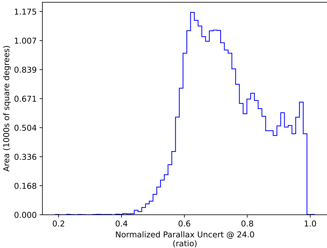
ddf_acor_sf20_lsf30_lsr20_v3.4_10yrs : Normalized Parallax Uncert @ 24.0
