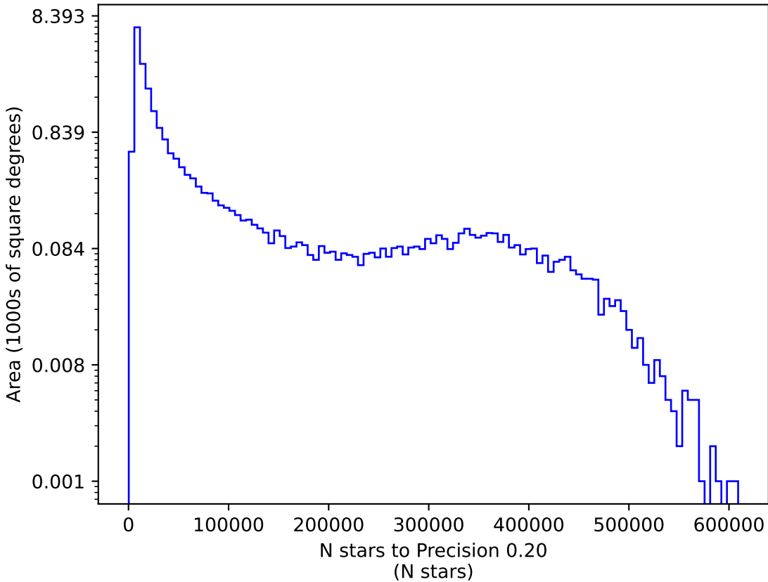
ddf_acor_sf20_lsf30_lsr20_v3.4_10yrs y: N stars to Precision 0.20
