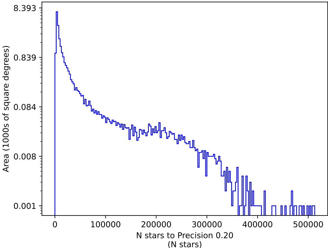
ddf_acor_sf20_lsf30_lsr20_v3.4_10yrs u: N stars to Precision 0.20
